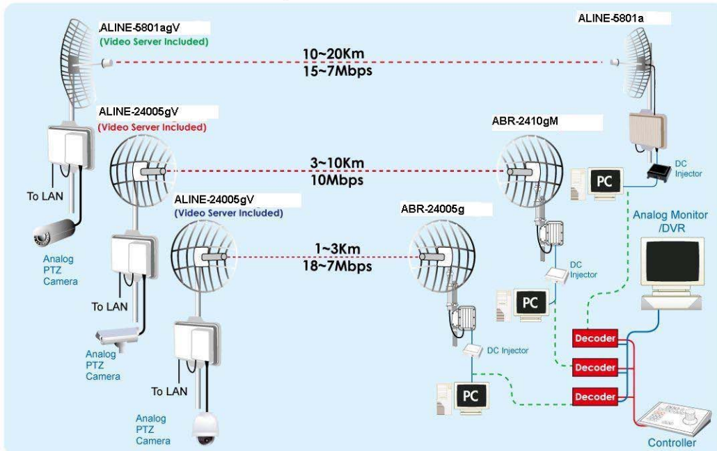
Point to Point Radio Link with Analog PTZ Camera, Transcoder and PC
